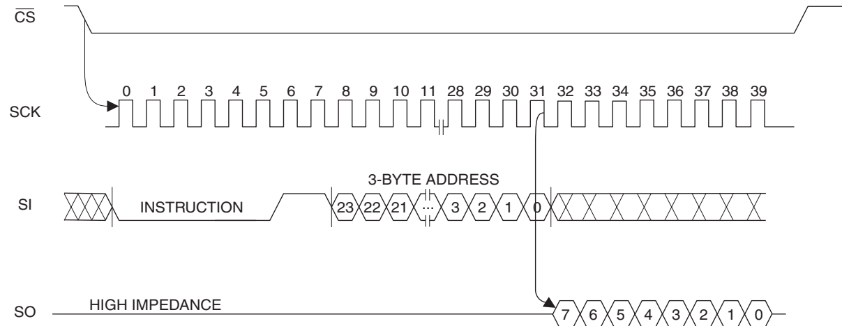
Figure 8. READ Timing
